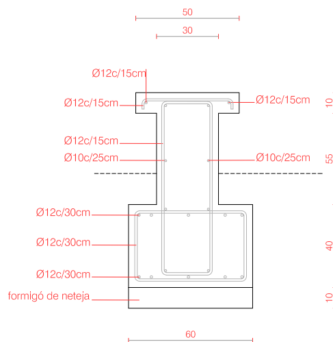
S2. DETALL ARMAT BANC
