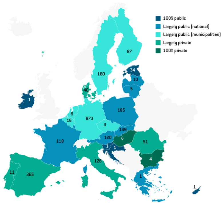
Figure 2: DSO (Distribution System Operators) ownership and number of DSOs per country
